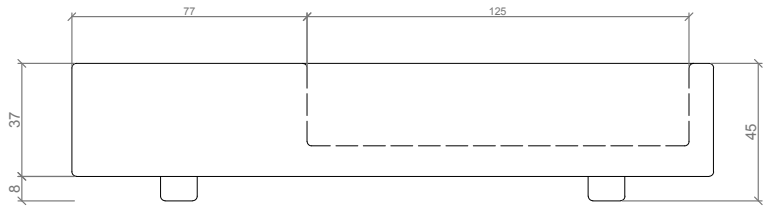
ALZADO / FRONT VIEW
