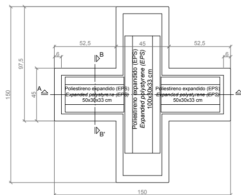
VISTA INFERIOR / BOTTOM VIEW
