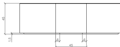
ALZADO / FRONT VIEW
